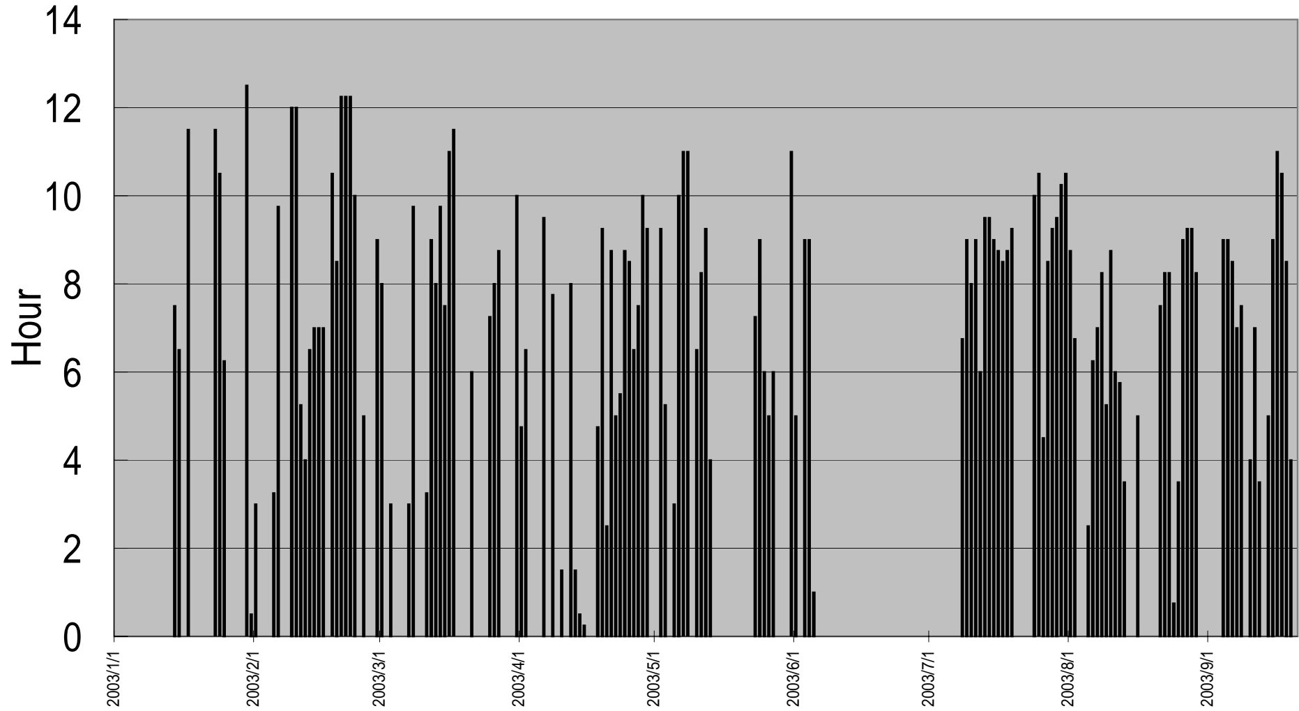
Lulin obs_time (20030114~20030920)
