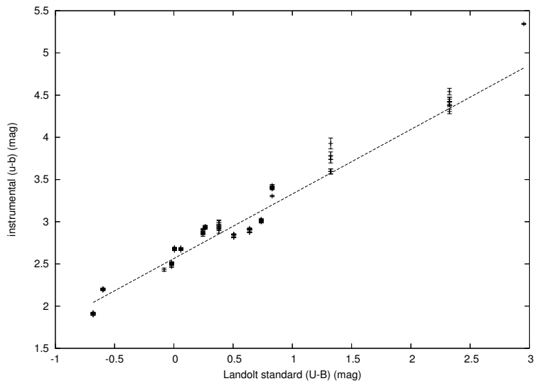
Fig. 12 The Landolt standard colors and the extinction corrected instrumental colors are plotted for (U - B) . The dotted straight line is the least-square fit of the data. The data were collected on 25 June, 2004.
