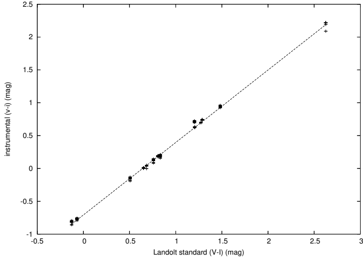
Fig. 15 Same as Figure 12, but for (V - I) .
