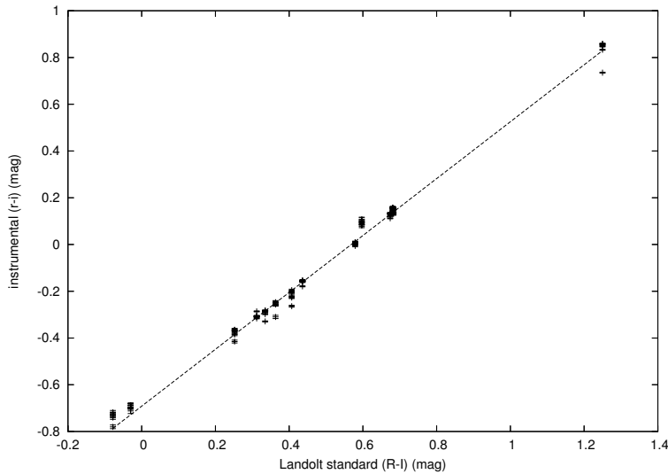
Fig. 16 Same as Figure 12, but for (R - I) .
